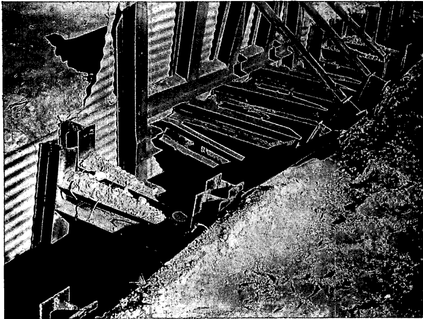
Fig. 6—Close-up view showing collapse of steel ramp wall after Dog shot.
